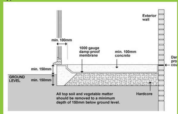
Typical solid floor detail
